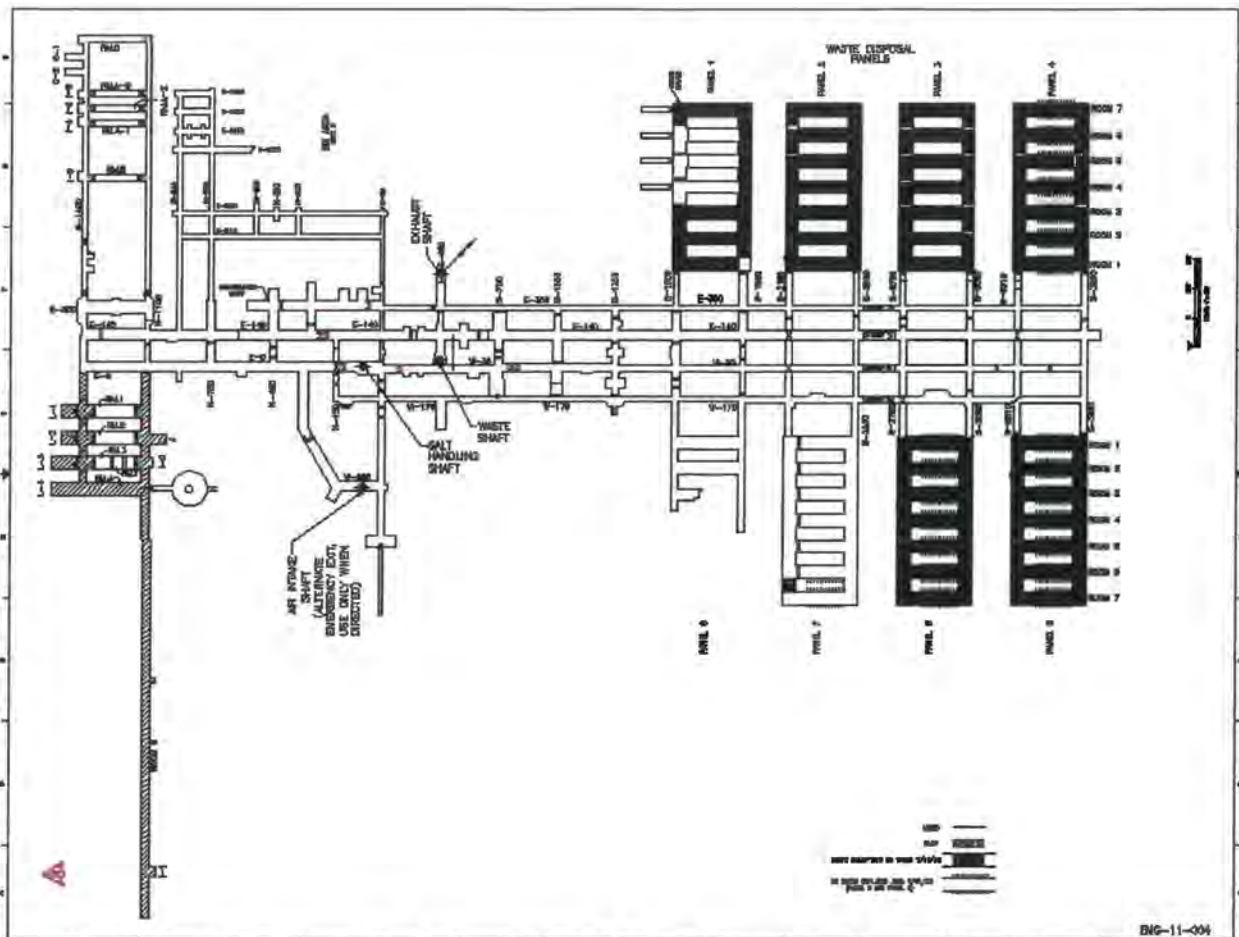
Figure 2.1. Configuration of the WIPP Underground for Geotechnical COMPs (after DOE 2016b; Reporting Period July 2014 through June 2015).
