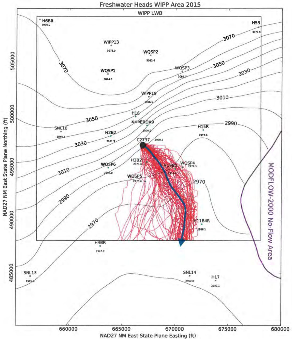
Figure 2.15. January 2015 modeled Culebra potentiometric surface of the immediate WIPP vicinity (DOE 2016b) generated using ensemble average distributed aquifer parameters from the SNL Culebra flow model used in CRA-2009 PABC (Kuhlman, 2010b). Particle trace from the center of the WIPP waste panels to the LWB for the January 2015 potentiometric is shown with blue arrow. Distribution of 100 particle traces from CRA-2009 PABC is shown with red lines. Culebra monitoring wells are indicated with green circles.
