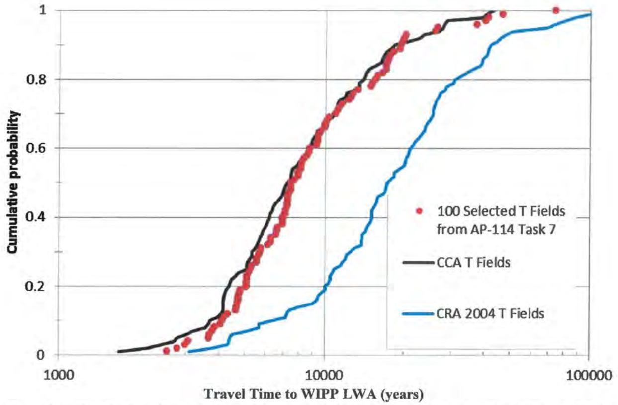
Figure 2.16. Distribution of Particle Travel Times from C-2737 (Center of Waste Panels) to WIPP LWB for CCA (black line), CRA-2004 (blue line), and CRA-2009 PABC (red dots). Figure from Hart et al. (2009).
