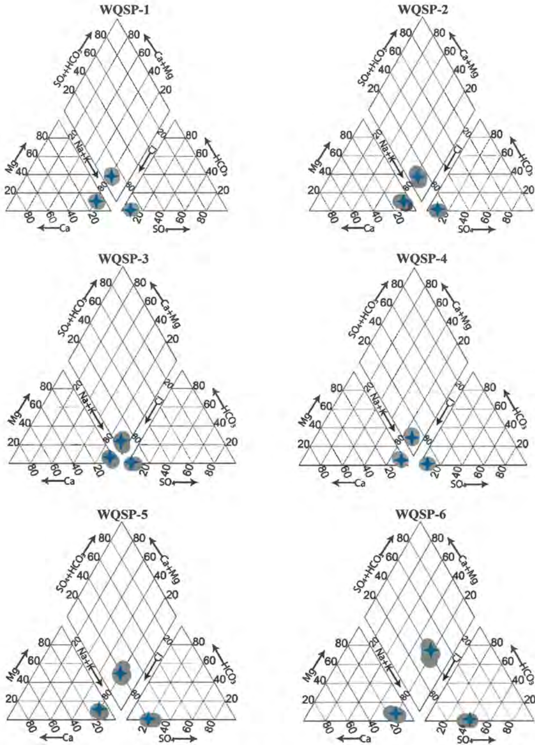
Figure 2.13. Piper diagrams of all data collected from WQSP-1 through WQSP-6. The plots show both historical data (gray areas) and results from Round 37 (blue "+").
